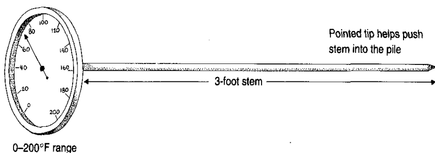
Figure 6.2 Dial thermometer for monitoring windrow/pile temperatures.
