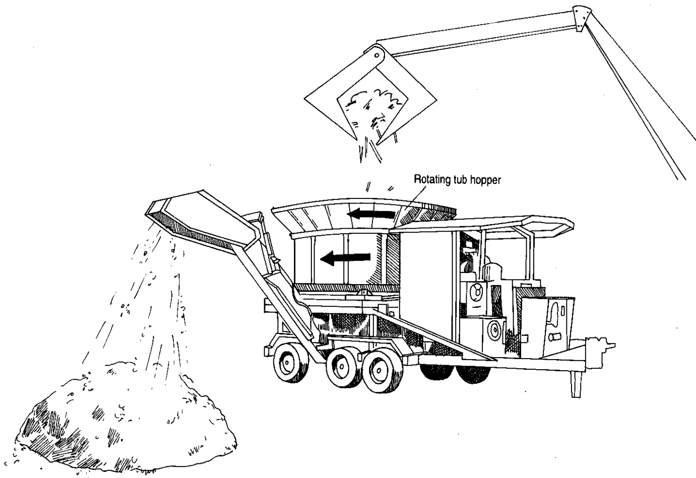
Figure 5.5 Tub grinder.
