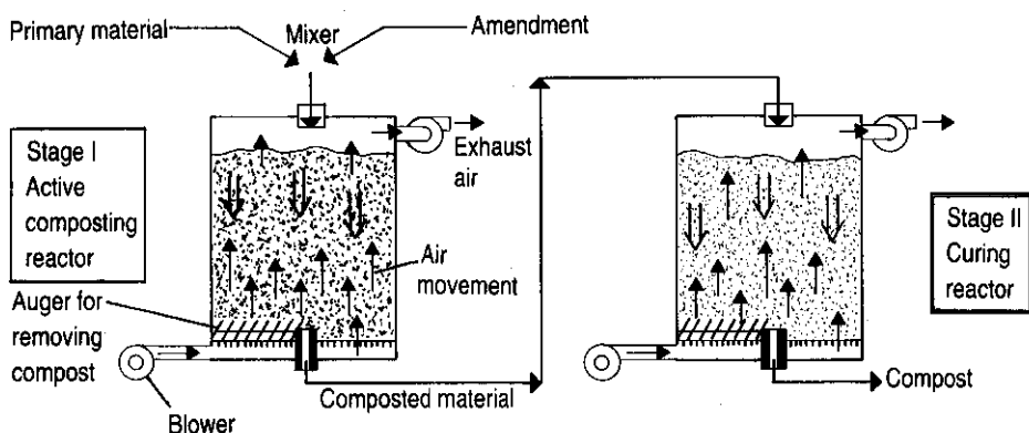
Figure 4.16 Silo composting system.
