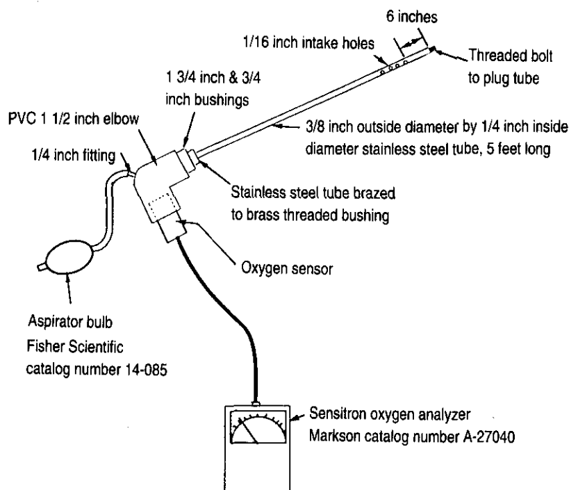
Figure 6.3 Oxygen-analyzing equipment.
