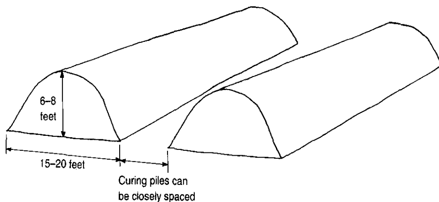
Figure 5.12 Curing pile dimensions.
